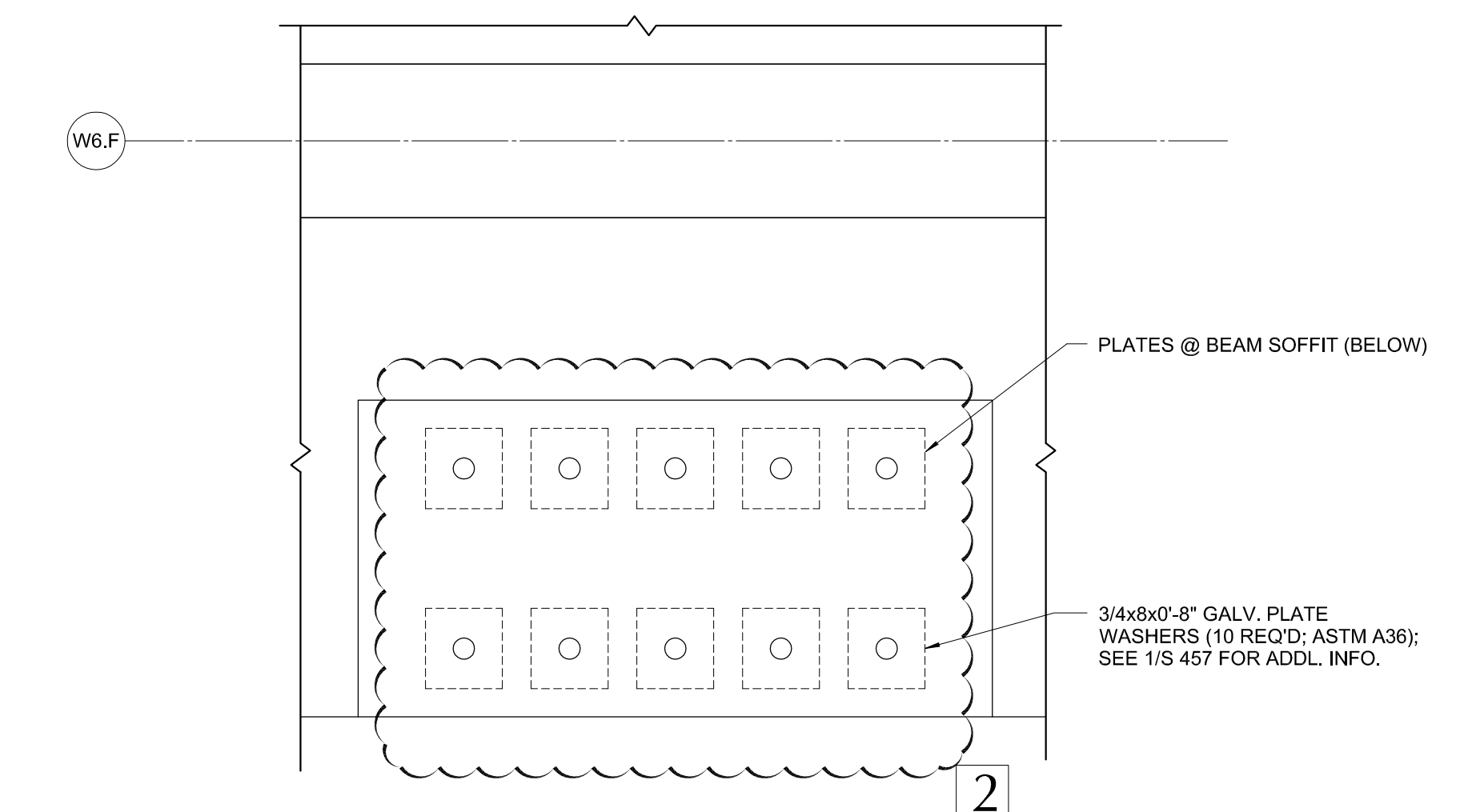
2 MOORING BOLLARD PLAN DETAIL SCALE: 3/4" = 1'-0"
