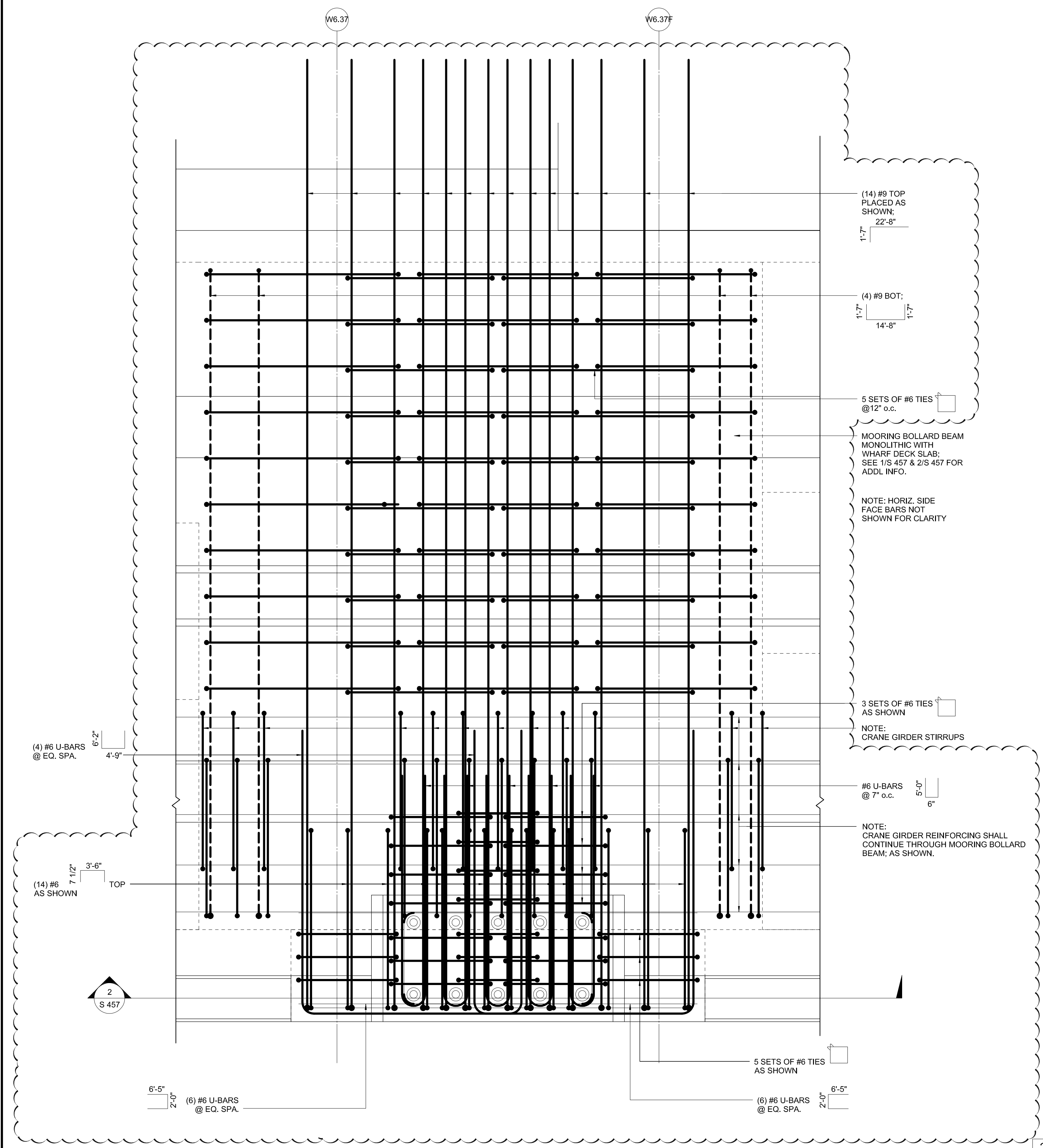
1 MOORING BOLLARD BEAM REINFORCING SCALE: 3/4" = 1'-0"
