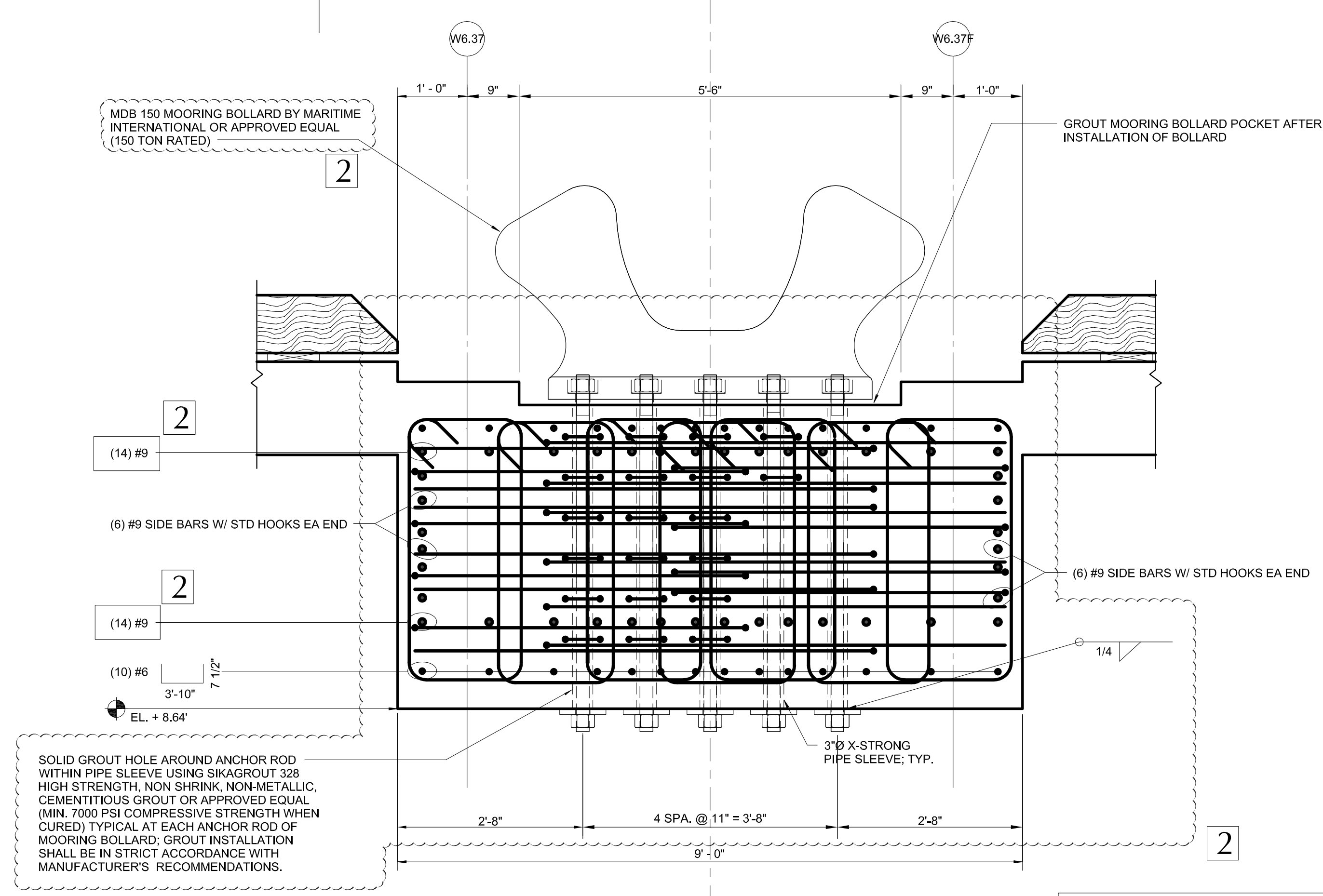
2 TRANSVERSE REINFORCING SECTION AT TYPICAL BOLLARD SCALE: 3/4" = 1'-0"
