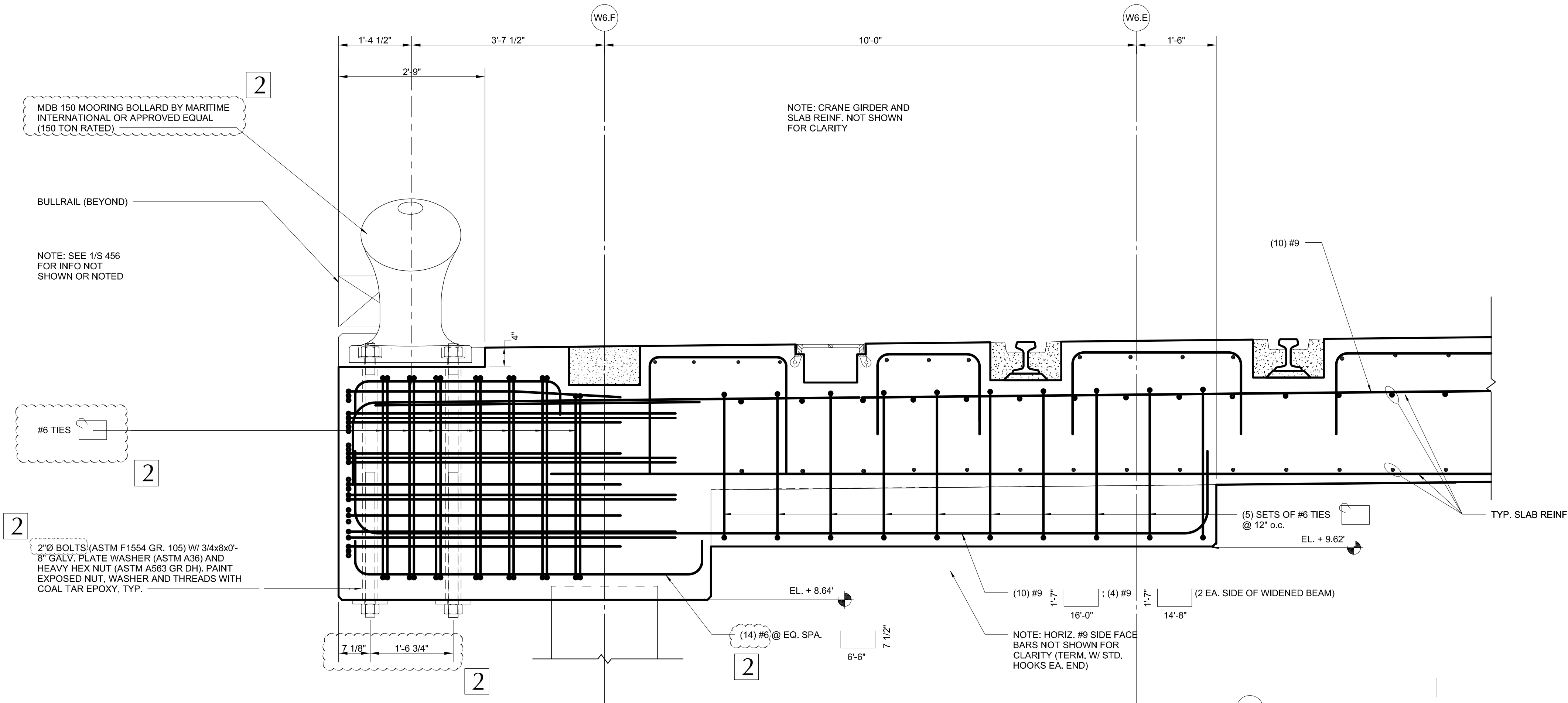
1 TYPICAL LONGITUDINAL SECTION AT MOORING BOLLARD BEAM SCALE: 3/4" = 1'-0"
