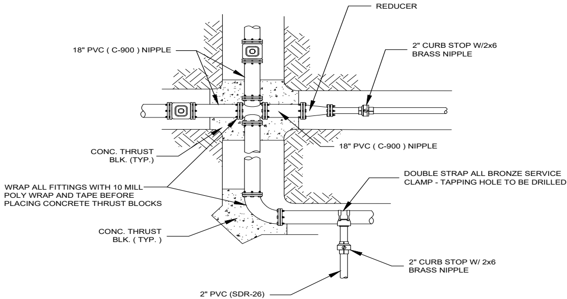
TYPICAL FITTINGS & CONCRETE THRUST BLOCK INSTALLATION
