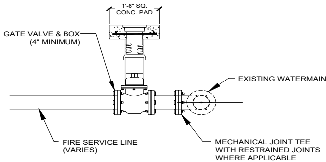
TYPICAL FIRE SERVICE LINE CONNECTION
