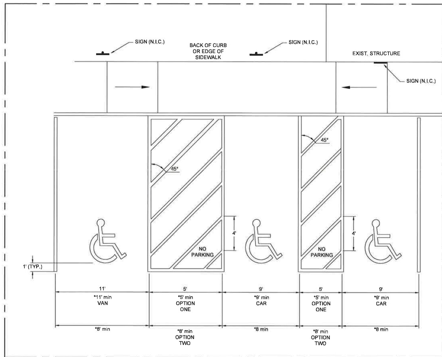
ENLARGED PLAN
