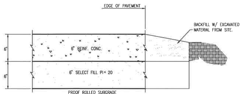
TYPICAL SECTION
