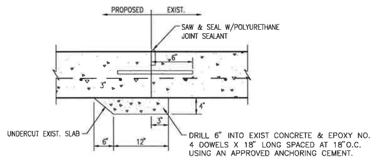
TYPE "E2" JOINT - EXIST. PAVEMENT
