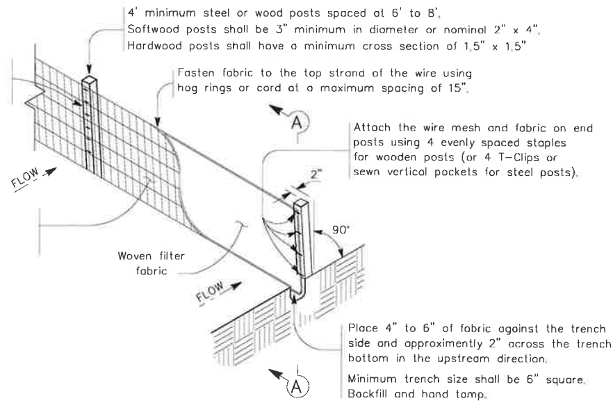
TEMPORARY SEDIMENT CONTROL FENCE
