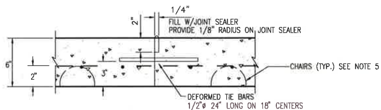
TYPE "E" "E1" CONSTRUCTION JOINT (TO BE USED AT END OF DAY OR UNEXPECTED DELAY)
